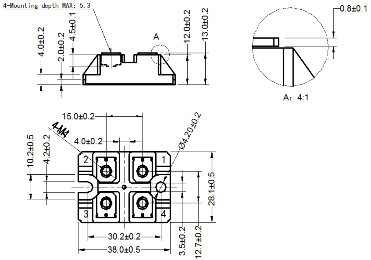
Dimensions in (mm) Figure 9. Package Outline
