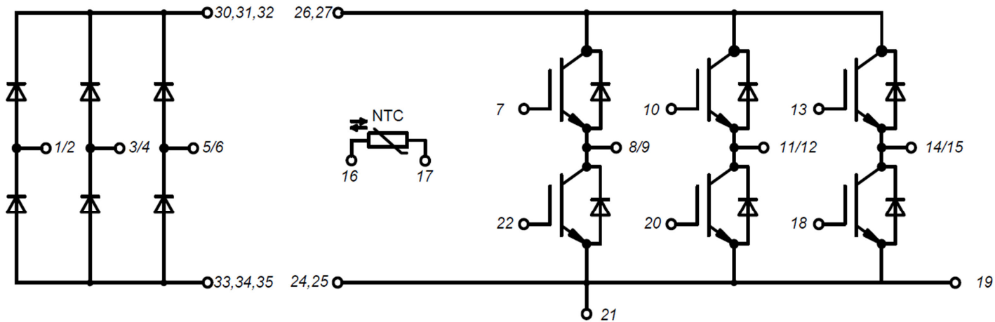
Figure 15. Circuit Diagram
