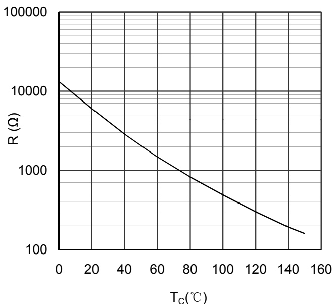
Figure 12. NTC Characteristics
