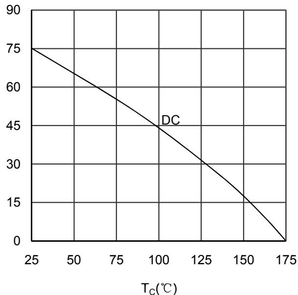
Figure 14. Forward current vs Case temperature Diode-inverter
