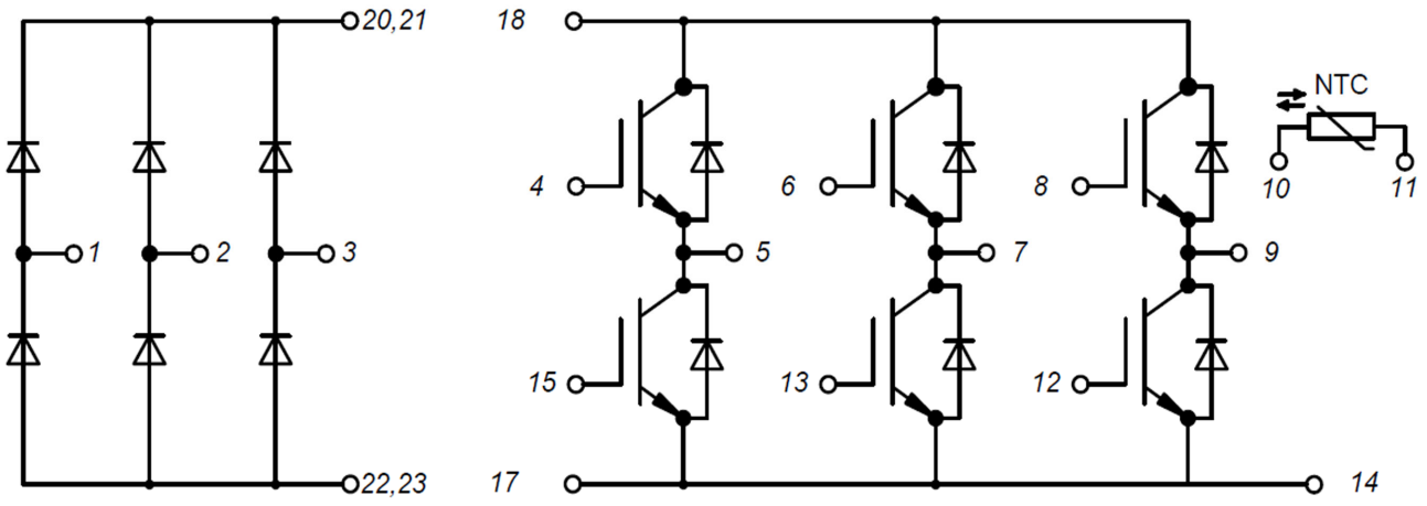
Figure 15. Circuit Diagram
