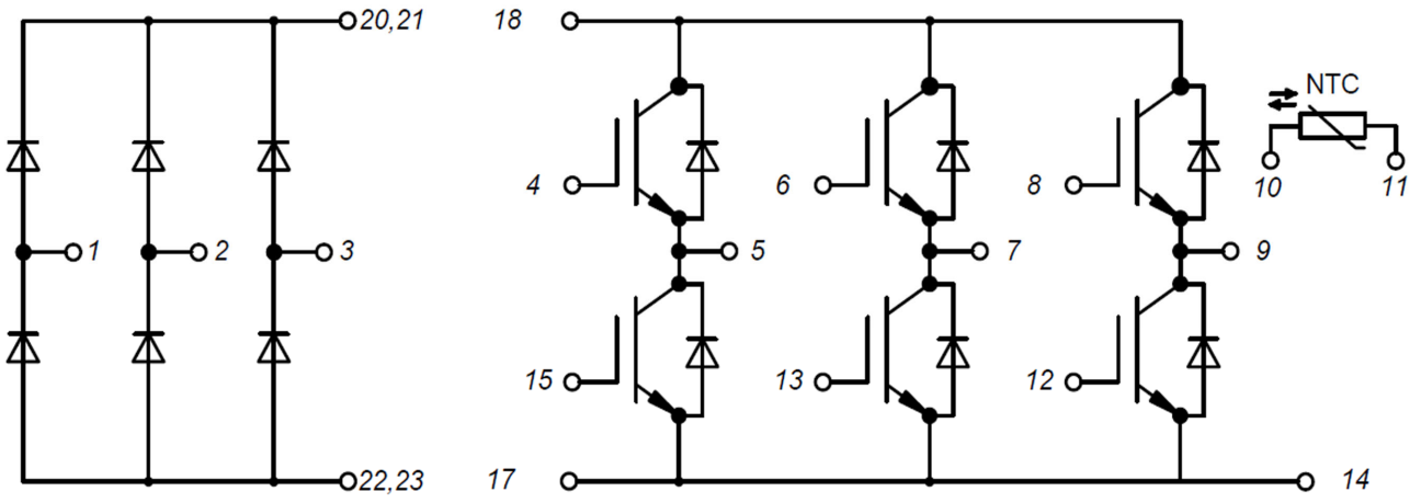
Figure 15. Circuit Diagram
