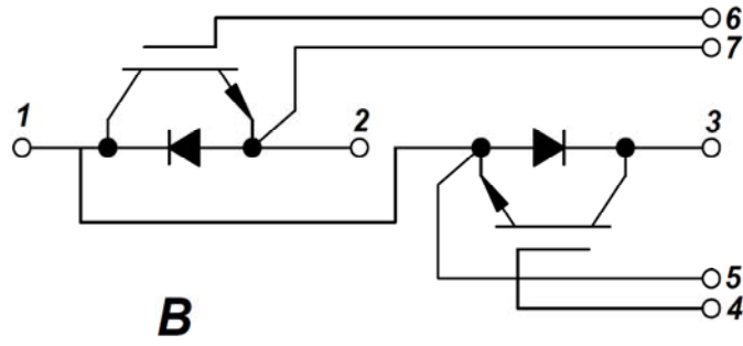
Figure 13. Circuit Diagram
