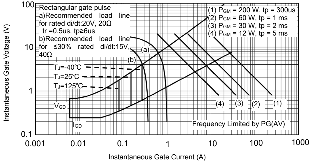
Figure 7. Gate Characteristics
