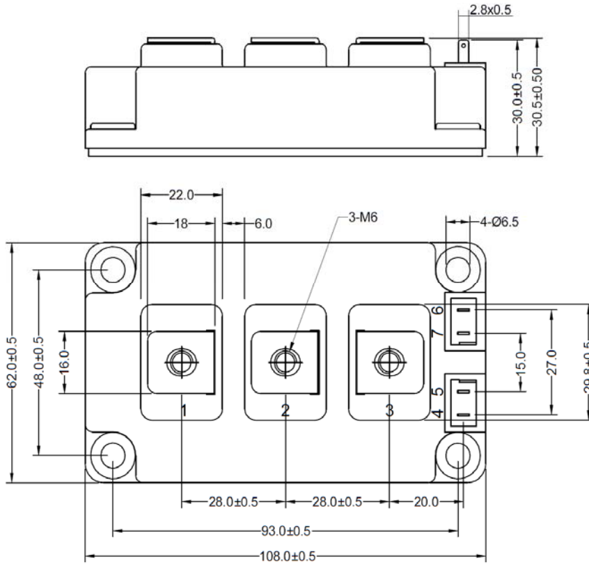
Figure 14. Package Outline
